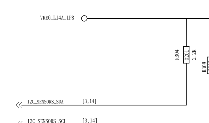
sensor I2C
