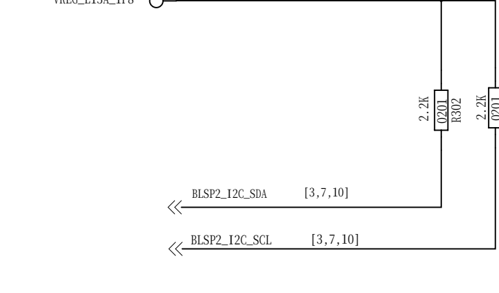
SMB I2C
