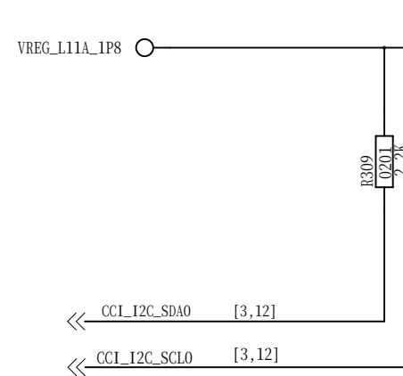
camera I2C
